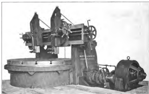
Fig. 4902. 84-Inch Tire Turning Mill. Betts Machine Co.
